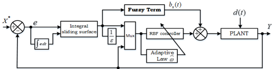
Figure 2. Detailed block-diagram of the RBF-Neuro-Fuzzy sliding mode controller
