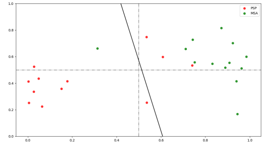
(b) 2-dimensional FDA followed by LR
