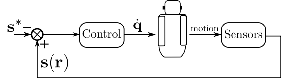
Fig. 1: Aural servo control scheme: a sensor-based approach links the motion of the robot to the sensor measurement \mathbf{s}(\mathbf{r}) in a feedback loop until the robot reaches a desired configuration characterized by a demanded measurement \mathbf{s}^* .
