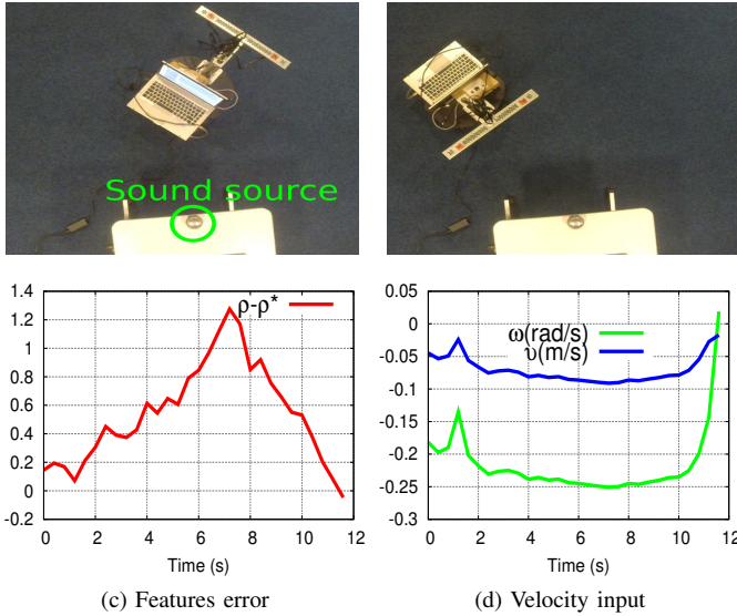
Fig. 6: The front-back ambiguity is inherently solved by the control scheme using ILD
