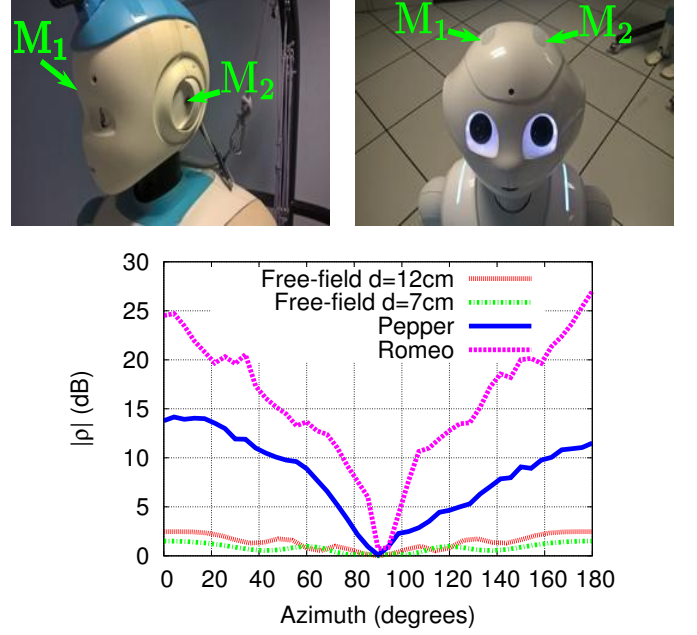
Fig. 12: ILD variation measurement on Romeo (top-left) and Pepper (top-right)
