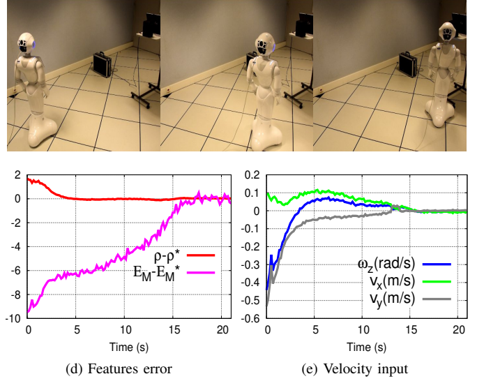
Fig. 15: Pepper approaches the sound source and reaches a pose satisfying \rho = \rho^* = 1 and E_M = E_M^* .
