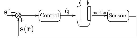
Fig. 1: Aural servo control scheme: a sensor-based approach links the motion of the robot to the sensor measurement s(r) in a feedback loop until the robot reaches a desired configuration characterized by a demanded measurement s^* .
