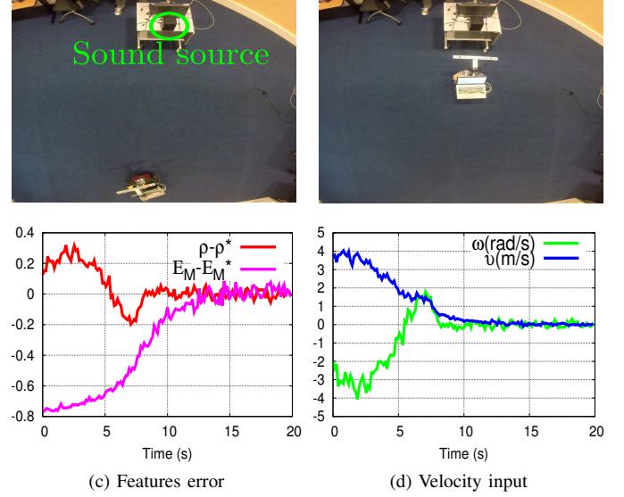
Fig. 9: A positioning task based on ILD and energy level measurement
