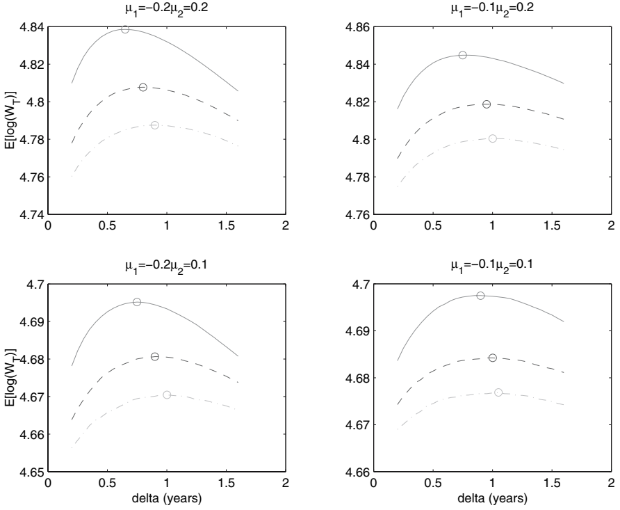
Fig. 2. Volatility and Optimal Moving Average Window Size: Plot of Expected Value of the Log of Terminal Wealth vs. Window size with T = 2 , \lambda = 2 , - \sigma = 0.1 , -- \sigma = 0.15 , and - . \sigma = 0.2 .
