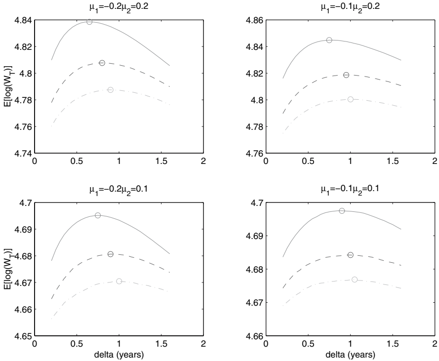
Fig. 2. Volatility and Optimal Moving Average Window Size: Plot of Expected Value of the Log of Terminal Wealth vs. Window size with T = 2 , \lambda = 2 , - \sigma = 0.1 , -- \sigma = 0.15 , and . \sigma = 0.2 .
