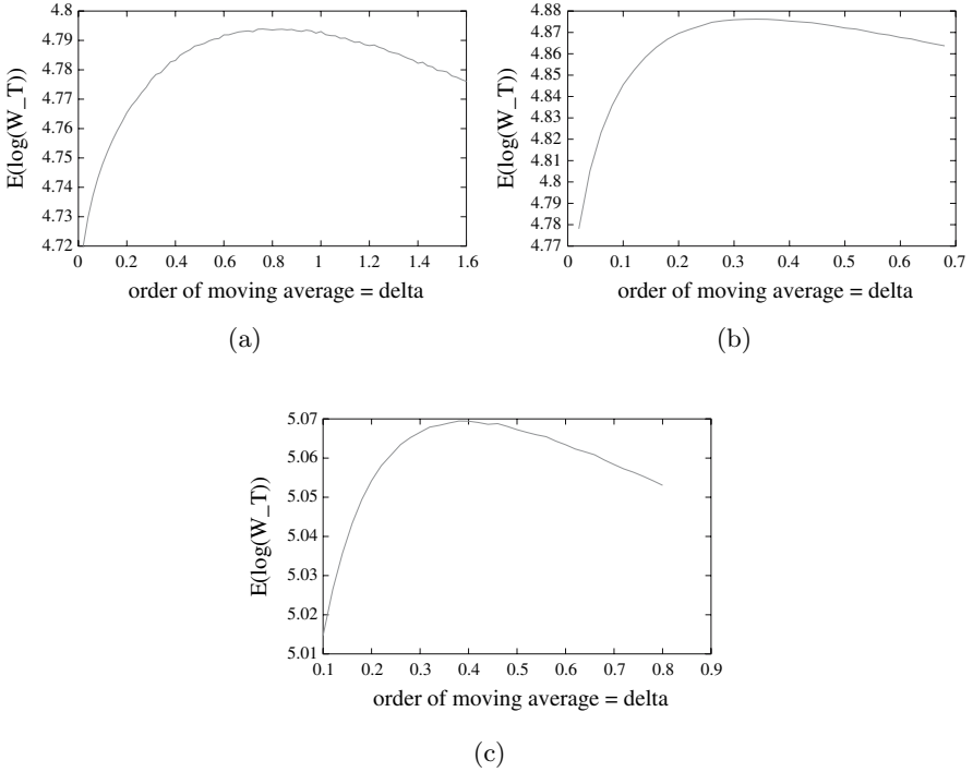
Fig. 1. \mathbb{E}(\log(W_T)) as a function of \delta .
