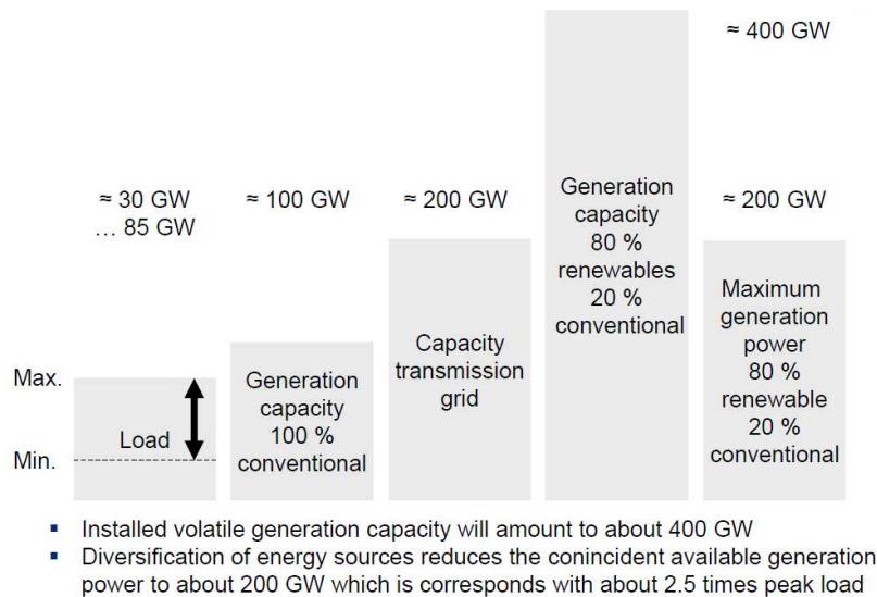
Fig. 1: Generation capacity required to achieve the 80 % renewable energy source target with respect to an annual electricity demand of about 600 TWh
