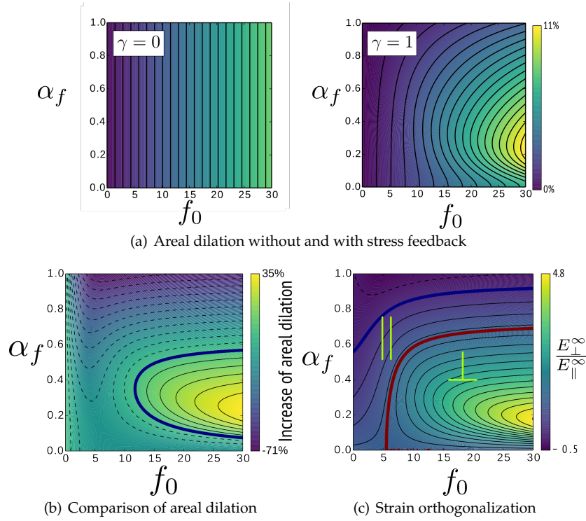
Fig. 4 The effect of stress feedback on elastic strain. Stress feedback confers nonlinear elastic properties to the material. Two noticeable effects are the effect of microfibril reorganization on areal expansion (that may differ relative to the isotropic linear case) and the strain and stress respective directions (that may be orthogonal). (a) Areal dilation ( \text{Tr}(E^{\infty}) ) \Delta_{\text{OFF}} without ( \gamma = 0 ) and \Delta_{\text{ON}} with ( \gamma = 1 , unit: 10^{-6} \text{ Pa}^{-1} ) feedback. In absence of feedback, dilation is a linear function of f_0 , which is not the case with feedback. (b) Relative variation (\Delta_{\text{ON}} - \Delta_{\text{OFF}}) / \Delta_{\text{OFF}} (in %) of areal dilation between a stress-responsive material ( \gamma = 1 ) and a non-responsive material ( \gamma = 0 ), as a function of f_0 (expressed in MPa) and stress anisotropy \alpha_f . Blue bold contour indicates level 0 ( \Delta_{\text{OFF}} = \Delta_{\text{ON}} ). (c) Ratio E_{\perp}^{\infty} / E_{\parallel}^{\infty} of strain (in the stress eigenbasis, where the basis vectors are sorted according to the descending order of eigenvalues) as a function of f_0 (expressed in MPa) and \alpha_f , with stress feedback. Main stress and strain are orthogonal iff E_{\perp}^{\infty} / E_{\parallel}^{\infty} > 1 ; domains labeled \perp and \parallel respectively indicate those where main stress and strain are orthogonal or collinear. Blue and red bold contours respectively indicate levels 0 (null orthogonal strain E_{\perp}^{\infty} ) and 1 (isotropic strain E_{\perp}^{\infty} = E_{\parallel}^{\infty} ). Parameters: c_0 (arbitrary), \gamma = 10^{-6} \text{ Pa}^{-1} , K_{\phi} = 1 (arbitrary), K_{\rho} = 1 \text{ mol} \cdot \mu\text{m}^{-3} , Y_f = 2 \text{ GPa} , \nu = 0.2 , Y = 0.2 \text{ GPa} .
