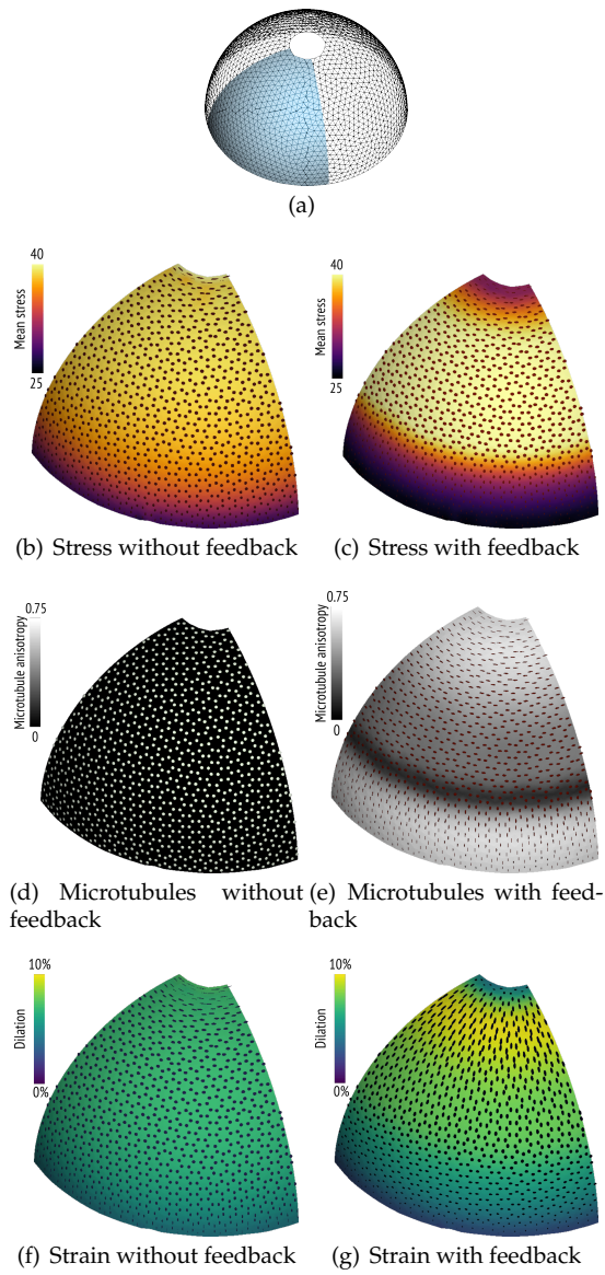
Fig. 7 Holed cap. Circular reorganization of microtubules allows to limit the effect of the breach by promoting radial expansion around the hole. (a) Original mesh and visualized cut (in blue). (b-c) Stress field. Heat map: mean stress f_0/2 (in MPa), elliptic representation of the tensor. (b) In absence of feedback, (c) with feedback. (d-e) Microtubule distribution. Heat map: microtubule anisotropy \alpha_\phi^\infty , ellipses: alignment tensor (see Appendix F). (d) In absence of feedback, (e) with feedback. (f-g) Strain field. Heat map: dilation \text{Tr}(E) . (f) In absence of feedback, (g) with feedback. Parameters: mesh characteristic dimension 100 \mu\text{m} (order of magnitude), turgor pressure P = 0.5 \text{ MPa} , \gamma = 2 \times 10^{-7} \text{ Pa}^{-1} , c_0 (arbitrary), K_\phi = 1 , K_\rho = 1 \text{ mol} \cdot \mu\text{m}^{-3} , Y_f = 20 \text{ GPa} , \nu = 0.2 , Y = 0.5 \text{ GPa} .
