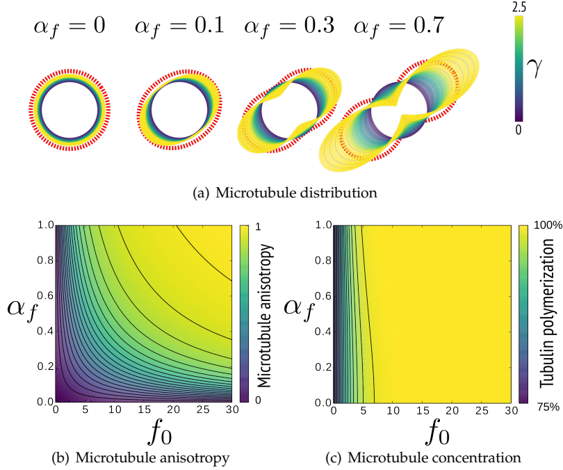
Fig. 3 Steady state of the microtubule distribution. Microtubules respond nonlinearly to stress anisotropy and amplitude. Microtubule anisotropy depends equally on both stress anisotropy and amplitude. (a) Visualization of the microtubule distribution \phi according to the stress anisotropy \alpha_f ( f_0 = 1 MPa) and the coupling coefficient \gamma . The red dashed line represents the polar distribution of forces f . (b) Anisotropy a_\phi^\infty of the microtubule distribution as a function of f_0 (expressed in MPa) and stress anisotropy \alpha_f with stress feedback. (c) Relative concentration of polymerized tubulin c_p^\infty/c_0 = \pi/2\phi_0^\infty/c_0 as a function of f_0 (expressed in MPa) and stress anisotropy \alpha_f with stress feedback. Parameters for (b-c): c_0 = 1 \text{ mol} \cdot \mu\text{m}^{-3} , \gamma = 10^{-6} \text{ Pa}^{-1} , K_\phi = 1 .
