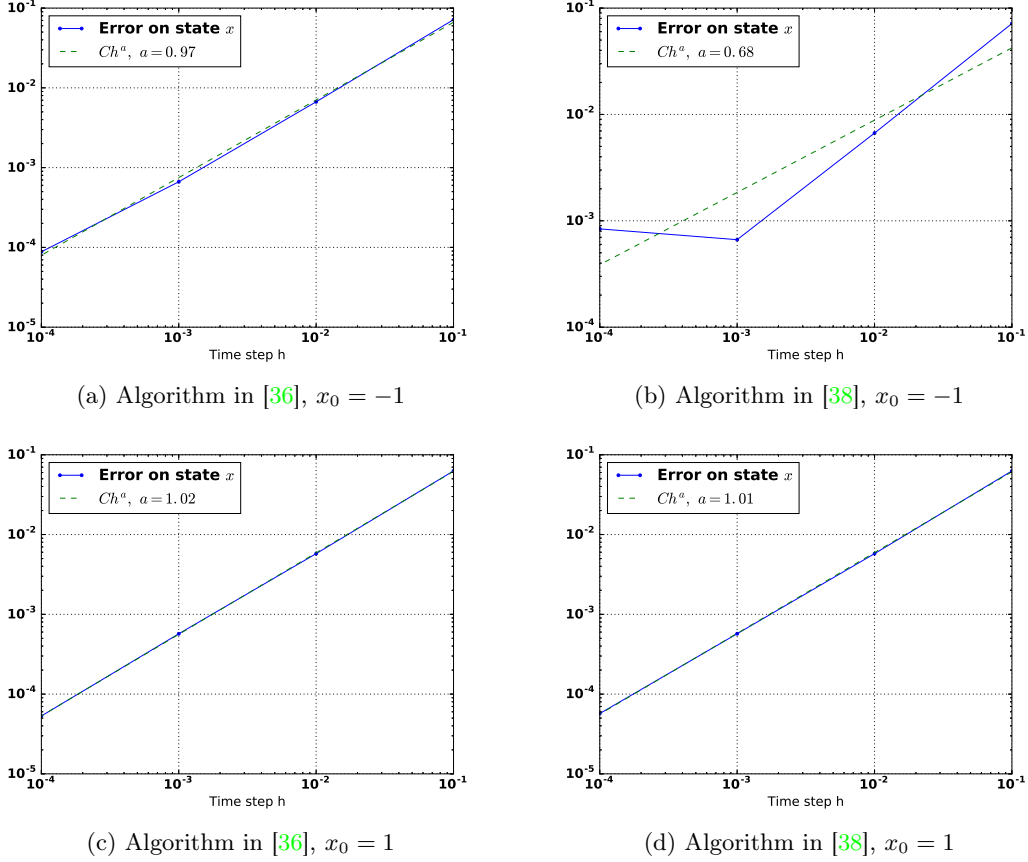
Figure 2: Error on state x when using Algorithms in [36] or in [38] with a = 3 , b = -0.5 , d = 1 , e = -2 , f = 3 , T = 1 and x_0 = -1 or x_0 = 1 in Example 1.
