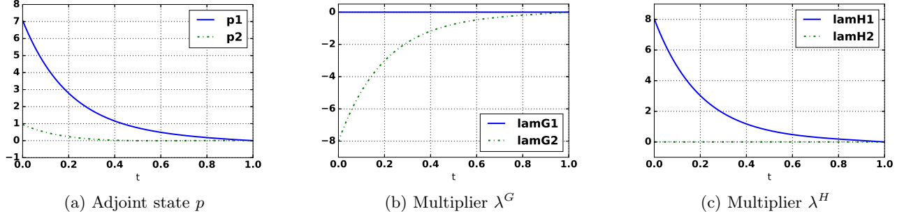
Figure 7: Computed multipliers for Example 3 using Algorithm in [35]. h = 10^{-3} .
