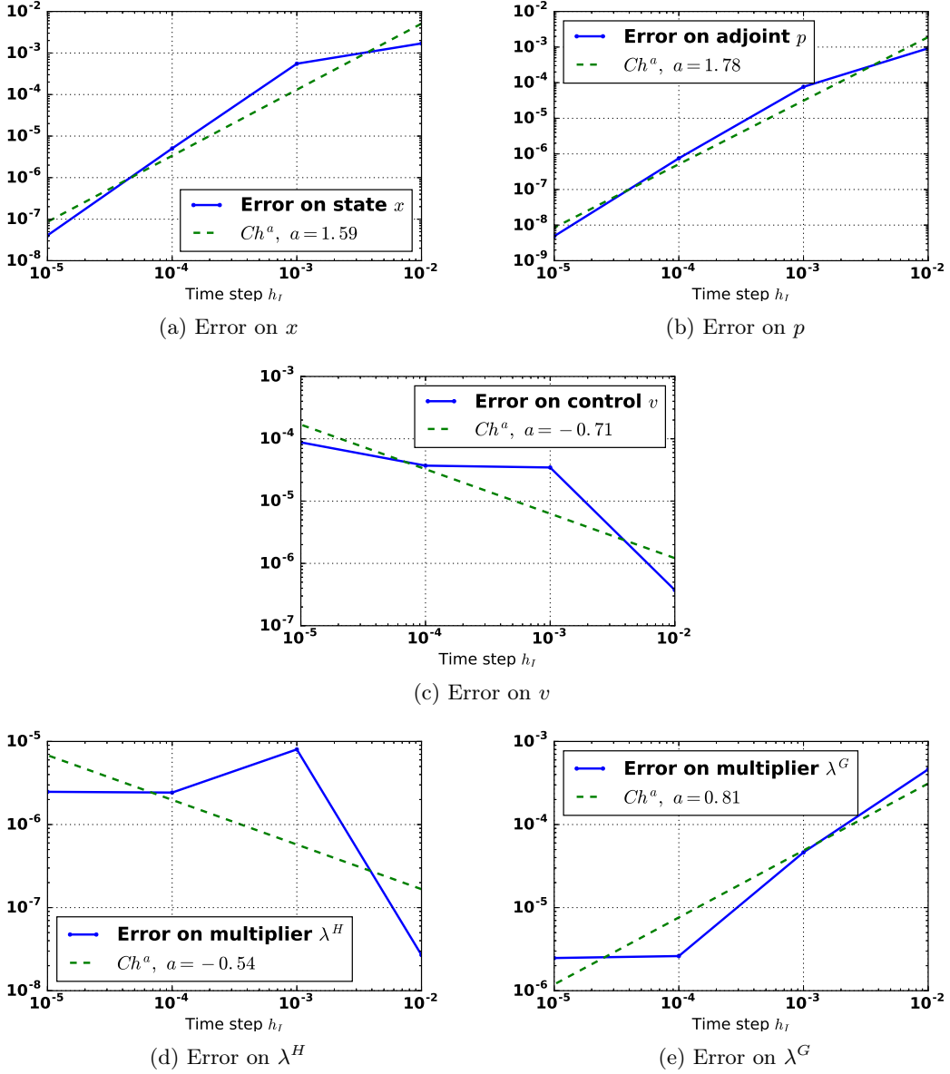
Figure 15: Errors with the Hybrid Approach for Example 1 with a = 3 , b = -0.5 , d = 1 , e = -2 , f = 3 , T = 1 and x_0 = 1 .
