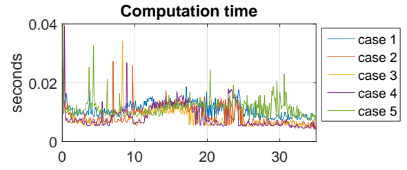
Fig. 11: Computation time
