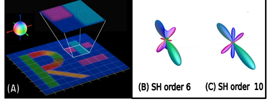
Fig. 1. Fiber ODF generation. (A) Simulated dataset shows the principle of super-voxel definition, adapted from [3]. The corresponding fiber ODF is reconstructed in (B) with pliODF technique while in (C) our approach improves the angular resolution.
