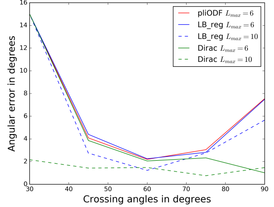
Fig. 3. Angular error: with L_{max} = 10 our method gives smallest error.
