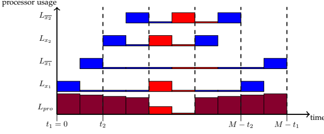
Figure 4: Example of a possible schedule for the instance \mathcal{J} associated to the formula x_1 \vee x_2 \vee \bar{x}_2 .
