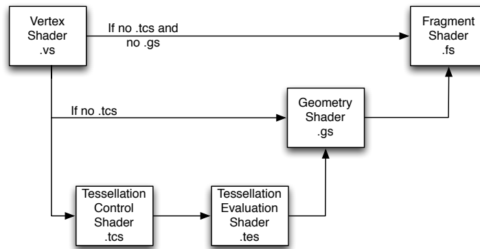
Fig. 2 Shaders used for the OpenGL graphic pipeline.
