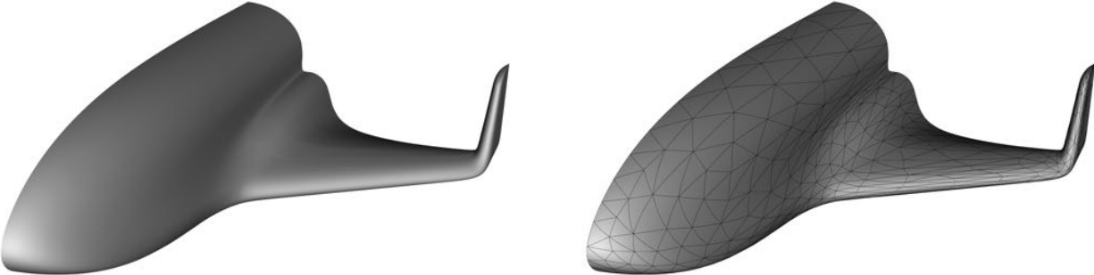
Fig. 6 Illsutration of an anisotropic \mathbb{P}_2 surface mesh approximating a shuttle NURBS with 2nd order elements.
