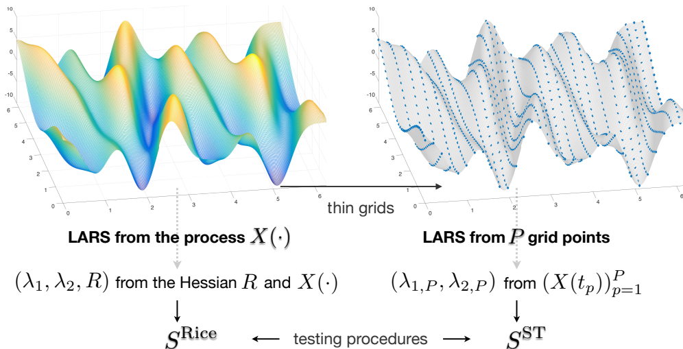
FIGURE 2. The grid-less approach uses the Hessian and the first two “knots” (\lambda_1, \lambda_2) of the “continuous” LARS to build the test statistics S^{\text{Rice}} . We compare it to the grid approach that builds a test statistics S^{\text{ST}} using the knots (\lambda_{1,P}, \lambda_{2,P}) computed from a P points grid discretization (X(t_p))_{p=1}^P of the continuous process X .
