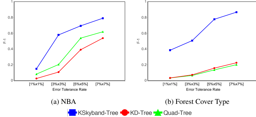
Fig. 7: F1 -measure of 3 techniques based on k -skyband tree, kd-tree and quadtree on the real datasets for k = 40 , \epsilon = 1.0 , and error tolerance rate ranges from 1% to 7% on each dimension.
