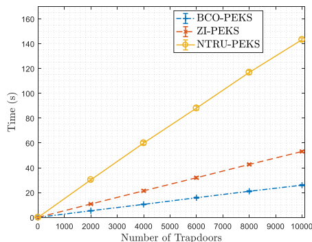
Fig. 4: Efficiency of Trapdoor algorithm
