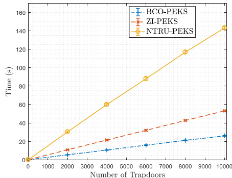
Fig. 4: Efficiency of Trapdoor algorithm
