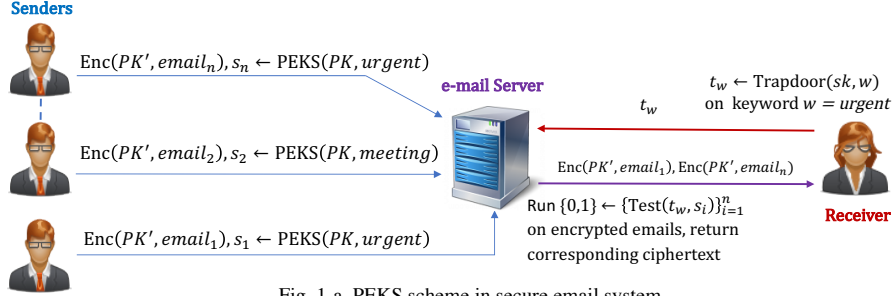
Fig. 1-a PEKS scheme in secure email system
