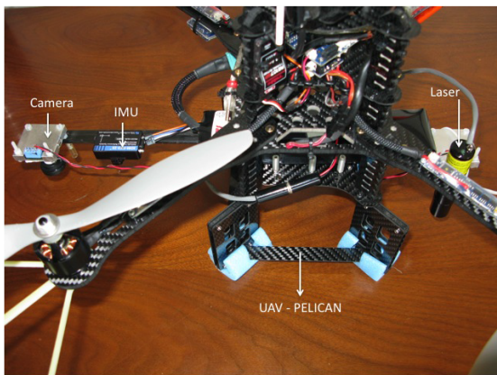
(a) Our system mounted on a Pelican UAV
