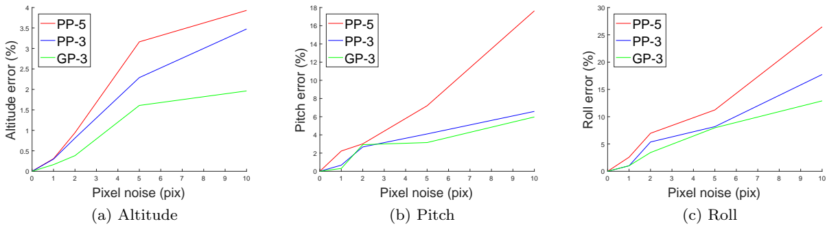
Fig. 7: Evaluation of the proposed algorithms under varying image noise.
