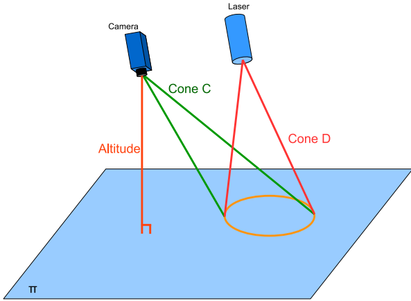
Fig. 1: Geometric representation of the laser/camera setup
