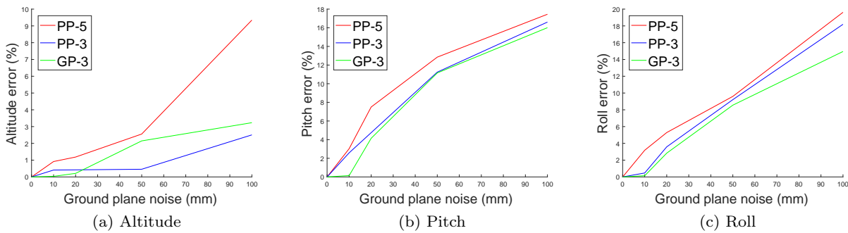
Fig. 11: Evaluation of the proposed algorithms under varying ground plane noise.
