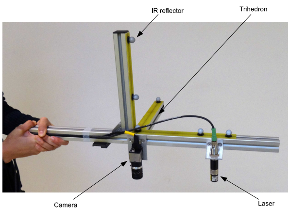
Fig. 12: The hand-held system used for the Vicon experiment
