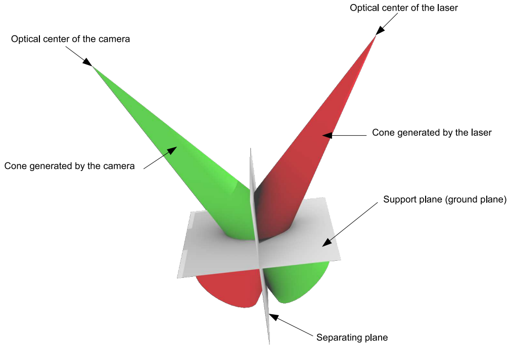
Fig. 2: Two cones generated by the same conic, intersect in general in a second conic.
