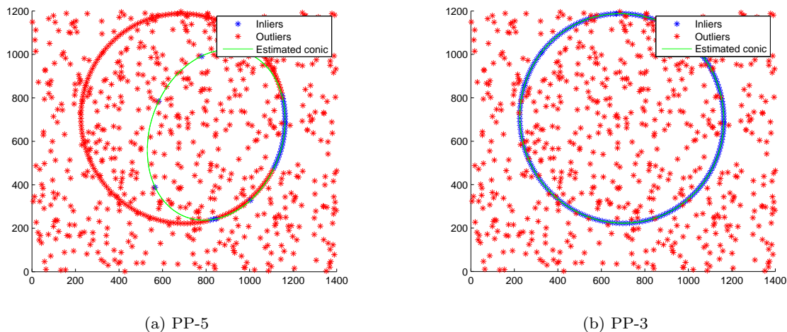
Fig. 8: The estimated conic using the PP-5 (a) and the PP-3 (b) algorithms. Outlier ratio = 75%, Number of RANSAC iterations = 100, RANSAC threshold = 0.01.
