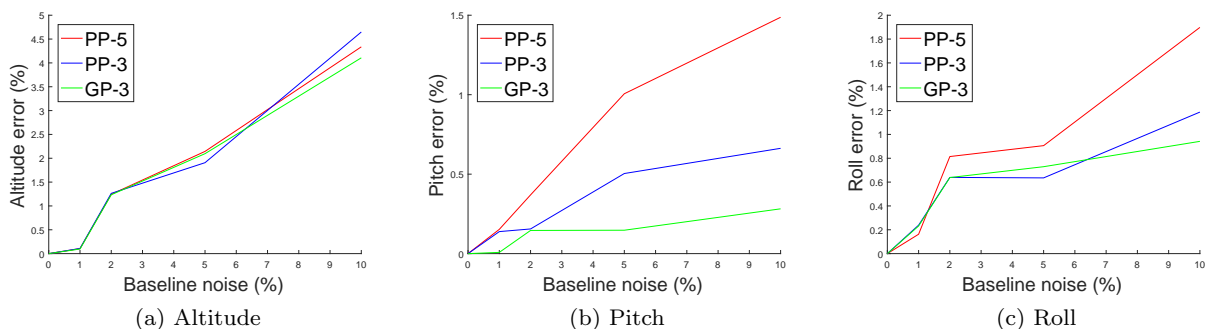
Fig. 10: Evaluation of the proposed algorithms under varying baseline noise.
