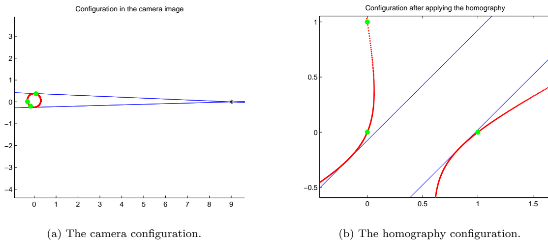
Fig. 4: Our problem in two configurations: in the camera image and after applying the homography. The 3 points selected to estimate \mathbf{c} are represented in green, the epipole in black, the two tangent lines in blue and the conic to be estimated in red. Note that on the right hand side, obtained by applying the projective transformation \mathbf{H} , the conic may not be an ellipse.
