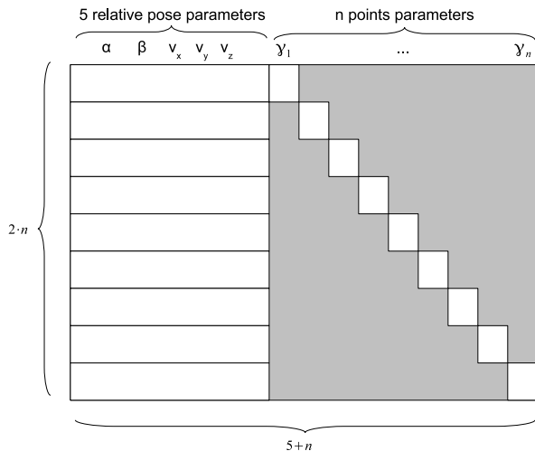
Fig. 6: Form of the Jacobian matrix for our calibration formulation consisting of 5 relative pose parameters and n points. Zero entries in the matrix are shown in gray.
