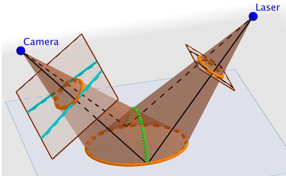
Fig. 3: Epipolar geometry of the camera and the projector. The black lines are tangents to the cones relative to an epipolar plane. Their projection into the camera image gives epipolar lines (in cyan) which must be tangent to \mathbf{c} . The green curve is the second intersection curve of the two cones, besides the ellipse on the ground plane (see text). This figure can be explored in 3D at https://www.geogebra.org/m/x3x62vRQ .
