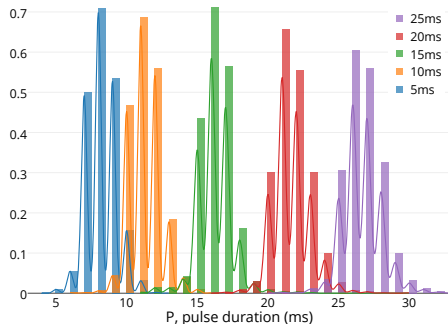
Fig. 8. Distribution of effective pulse duration for different configured pulse duration values.
