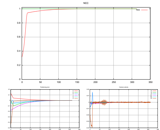
Fig. 9. Positioning task with respect with various metallic tools. A ring-light is mounted around the camera. Light is then moving.
