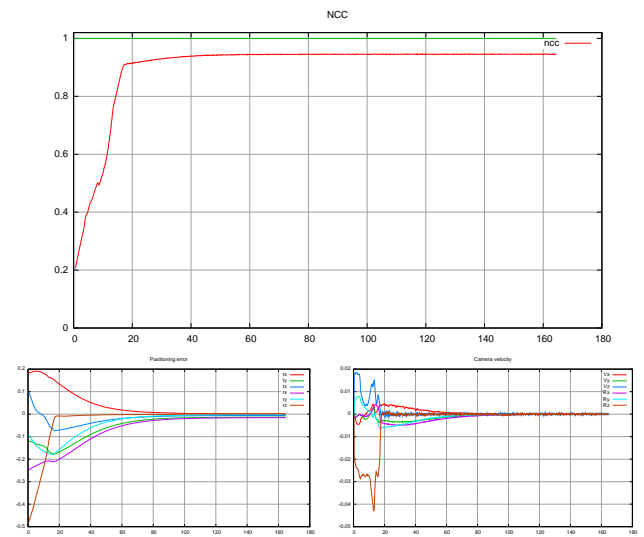
Fig. 7. ZNCC based visual servoing with important lighting variations (a) ZNCC criterion (b) positioning error (in cm and rad) (c) camera velocities in cm/s and rad rad/s
