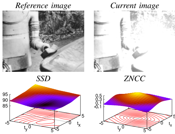
Fig. 2. Robustness of the cost functions with respect to global illumination variations.
