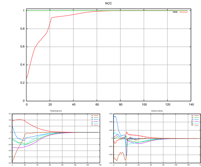
Fig. 5. ZNCC based visual servoing on a 3D scene (a-b) initial and desired image acquired by the camera. (c-d) initial and final error (that is \mathbf{I} - \mathbf{I}^* ) (e) ZNCC criterion (f) positioning error (in cm and rad) (g) camera velocities in cm/s and rad rad/s
