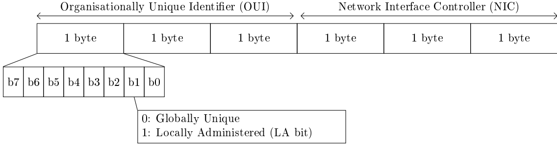
Figure 1: MAC address format.
