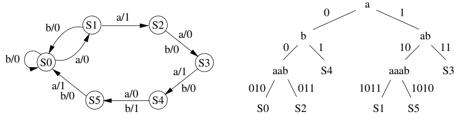
Fig. 1. FSM M_0 and a splitting tree T for it
