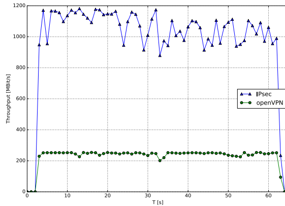
Fig. 2: Maximum Platform Throughput achieved by IPsec and openVPN
