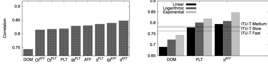
Fig. 3: Expert models: Impact of (a) explanatory QoS metric x for the f(\cdot) = \text{IQX} hypothesis and (b) combined impact of metric x and mapping function f(\cdot)
