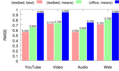
Fig. 8: Predictor evaluation.
