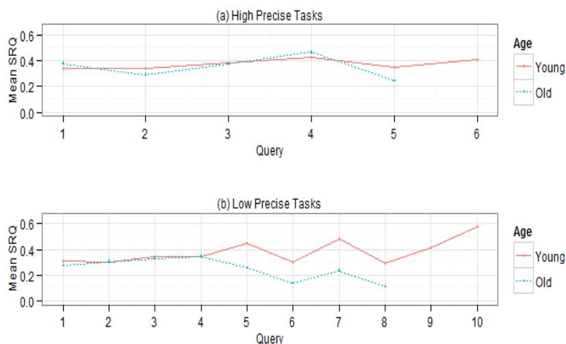
Fig. 5. Mean semantic relevance of queries with target at each reformulation cycle for (a) high precise and (b) low precise tasks
