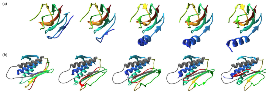
Fig. 9: (a) Collagenase: Steric clashes occur in the formation of the dark blue helix loop. (b) Spindle Assembly Checkpoint Protein: steric clashes occur in the formation of the dark blue helix and the motion of the red loop.
