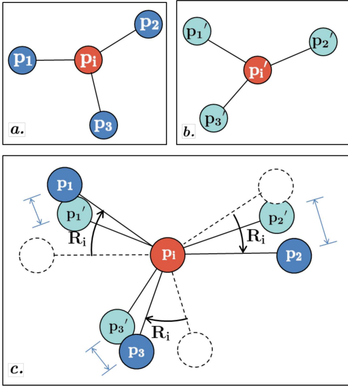
Fig. 4: The local ARAP rotation that maximizes rigidity. a. The initial cell. b. The target cell. c. The optimal rotation \mathbf{R}_i minimizes the sum of the rotated \|\mathbf{p}_j - \mathbf{p}'_j\|^2 distances (arrow bars), after aligning the cells such that \mathbf{p}_i = \mathbf{p}'_i .
