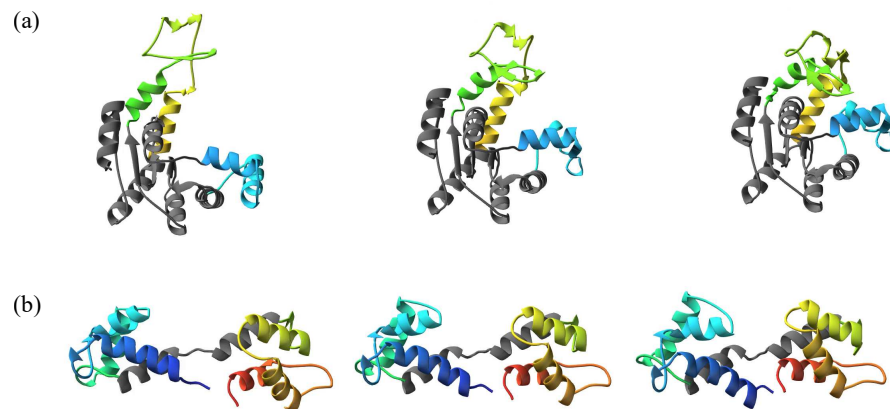
Fig. 7: Open-to-close motions in the colored parts of (a) Adenylate Kinase. (b) Calmodulin.
