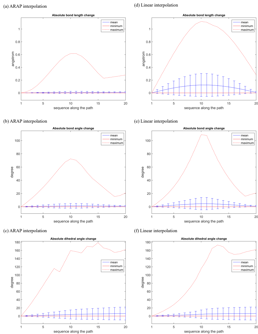
Fig. 5: Statistics of absolute changes in bond length, bond angle and dihedral angle for 5'-Nucleotidase. Results from ARAP interpolation for (a) bond length, (b) bond angle, (c) dihedral angle. Results from linear interpolation for (d) bond length, (e) bond angle, (f) dihedral angle.
