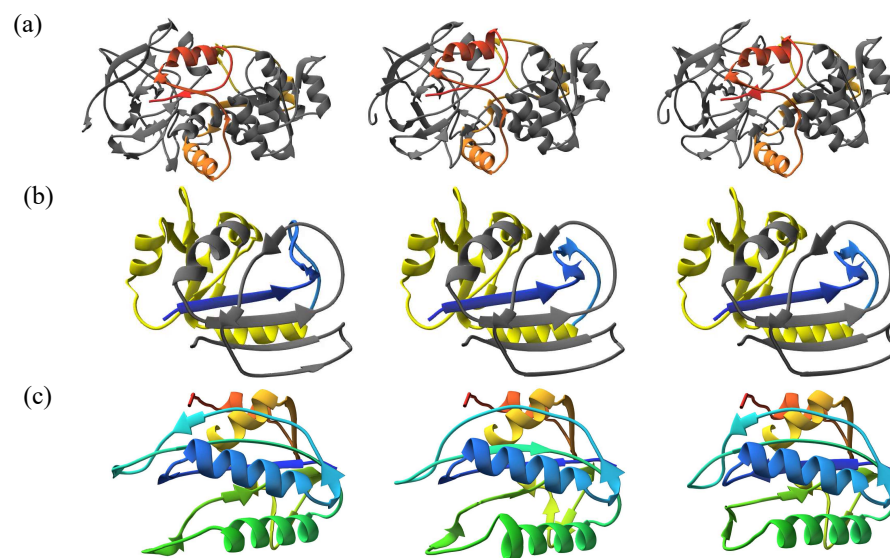
Fig. 8: Shear motions. (a) Alcohol Dehydrogenase: shear motion of the colored part compared to the static grey part. (b) Dihydrofolate Reductase: shear motion of the blue strand of the beta sheet. (c) Pyrophosphokinase: shear motion of the green helix and the light blue loops.
