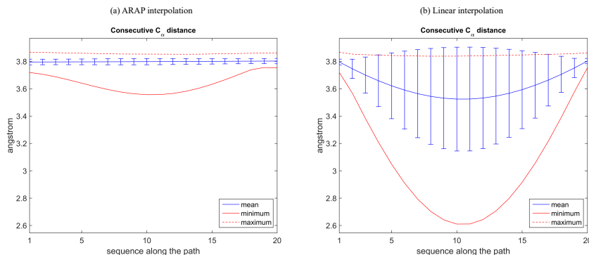
Fig. 6: Statistics of Consecutive C_\alpha distances for 5'-Nucleotidase from (a) ARAP interpolation, (b) Linear interpolation.
