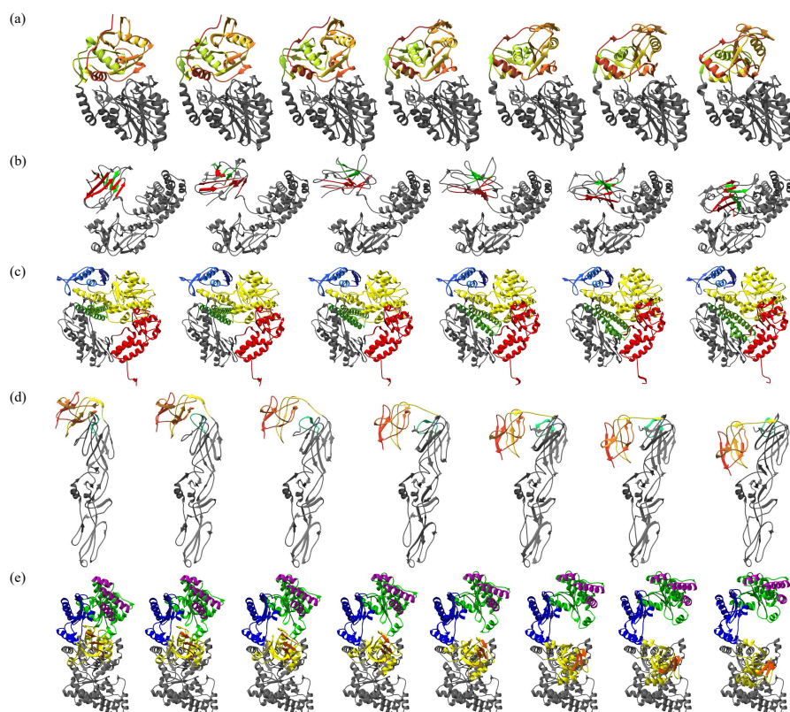
Fig. 10: Motion of (a) 5'-Nucleotidase: Rotation of about 90^\circ of the colored part can be detected by paying attention to the red helix. (b) Diphtheria Toxin: Rotation of about 180^\circ of the colored part can be detected by observing the beta sheets, i.e. the red sheet goes behind the green one in the final picture compared with the first. (c) DNA Polymerase: Closing motion of the green helices. (d) Dengue 2 Virus Envelope Glycoprotein: The closing motion of the red and yellow domains by rotation. The small light blue loop also rotates by 180^\circ . (e) Pyruvate Phosphate Dikinase: The opening motion accomplished by the green-purple domain and the yellow-orange domain. Rotation of 90^\circ of the yellow domain can be seen clearly by the orientation of the orange arrows. Rotation of the green-purple domain is smaller.
