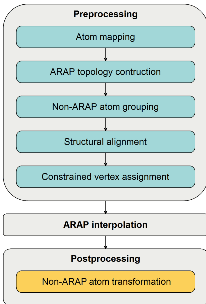
Fig. 1: Global framework to generate molecular paths from an initial to a target conformation using the ARAP interpolation method.
