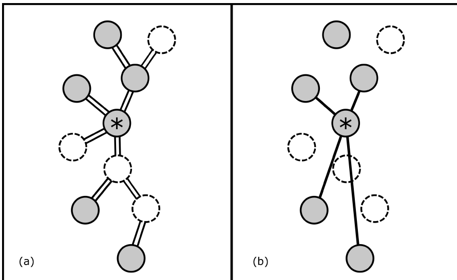
Fig. 2: Example of ARAP connectivity construction starting from the ARAP atom marked with a star. ARAP atoms are grey, while non-ARAP atoms are white. (a) The initial molecular topology. (b) ARAP edges created from the marked ARAP atom and represented by bold lines. When the connect procedure stops for the marked atom, the top-left ARAP atom is not connected, since its connection to the marked atom passes through another ARAP atom.
