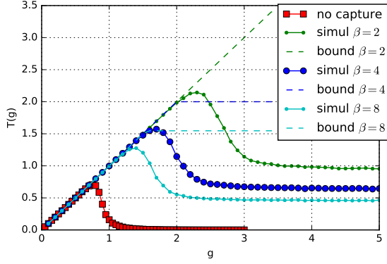
Fig. 4: Impact of capture threshold \beta on throughput
