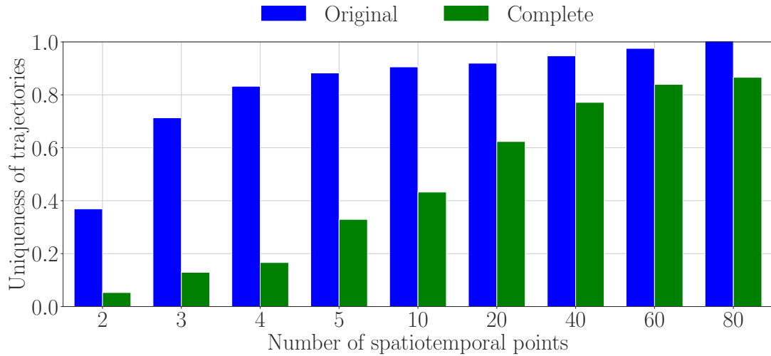
Figure 10: Revisited results from [5]. Ratio of trajectories with uniqueness |U| = 1 for a number of spatiotemporal points in the abscissa, for original (left) and complete (right) trajectories.
