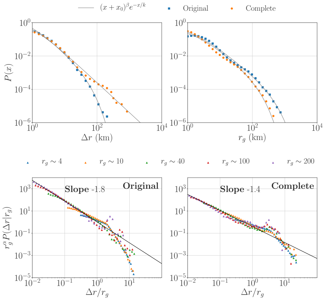
Figure 9: Revisited results from [3]. Distributions of travel distance \Delta r , radius of gyration r_g , and conditional travel distance \Delta r (with respect to \Delta r/r_g ) for original and complete trajectories.
