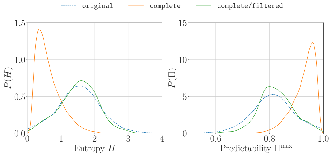
Figure 11: Revisited results from [4]. Distributions of the entropy and maximum theoretical predictability derived with (i) the incomplete original CDR-based trajectories of 8,000 users filtered with the method in [4], (ii) the complete trajectories of all 1.7 million users, and (iii) the complete trajectories of the same 8,000 users considered in the first case.
