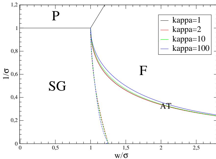
Fig. 2: Phase diagram in absence of bias and with a finite number of modes, with Gaussian distributions for u and v . The dotted line separates the spin glass phase from the ferromagnetic phase under the replica symmetry hypothesis. The RS phase is unstable on the left of the AT line. The influence of \kappa on the AT and (SG-F) lines is shown. In all cases the hypothetical SG-F line lies well inside the broken RS phase.
