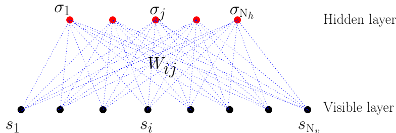
Fig. 1: RBM.
