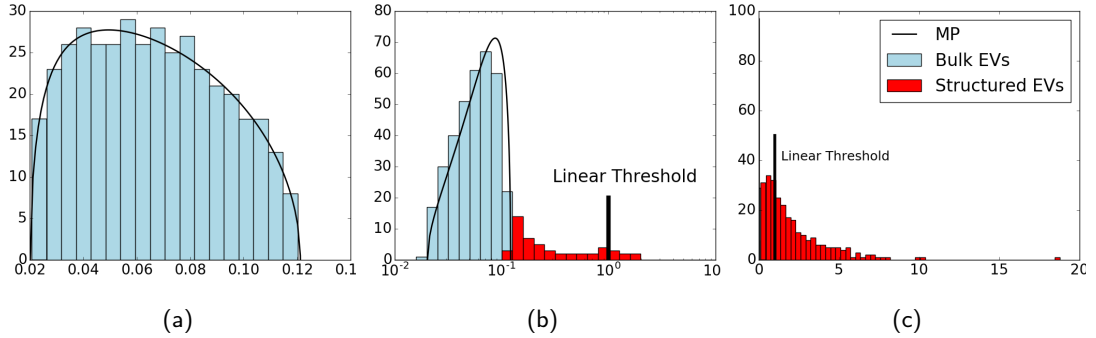
Fig. 8: (a) Singular values distribution of the initial random matrix compared to Marchenko-Pastur law. (b) With the training we can see some singular values strengthening and overcoming the threshold set by the Marchenko-Pastur law. (c) Distribution of the singular values after a long training: we can see many outliers spread above threshold and a spike of below-threshold singular values near zero.
