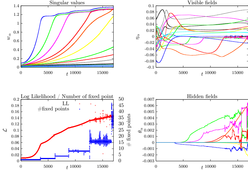
Fig. 5: Predicted mean Evolution of an RBM of size (N_v, N_h) = (1000, 500) learned on a synthetic data set of 10^4 samples of size N_v = 1000 obtained from a multi modal distribution with 20 clusters randomly defined on a submanifold of dimension d = 15 . The dynamics follows the projected magnetization in this reduced space with help of 15 modes. We observe a kind of pressure on top singular values from lower ones.
