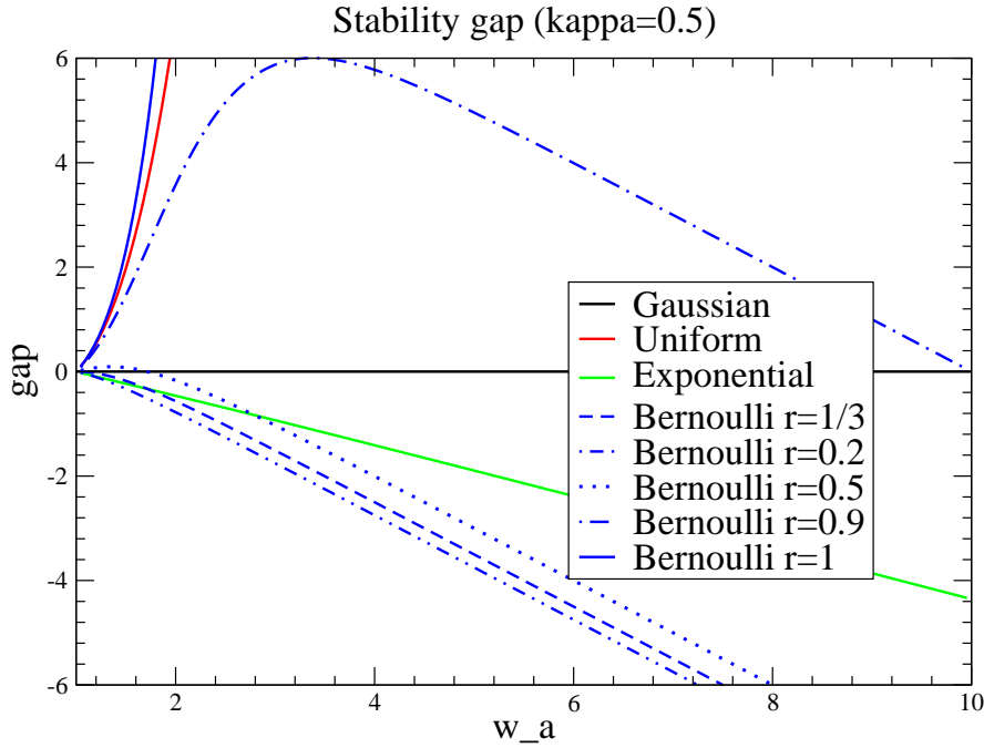
Fig. 3: Stability gap defined as \Delta w_\alpha as a function of w_\alpha for a fixed point associated to a mode \beta , corresponding to various distributions.
