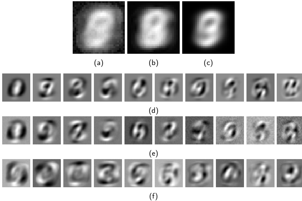
Fig. 9: (a) First mode learnt by the RBM with the external visible field initialized as a null vector. (b) External visible field initialized on the empirical mean. (c) First principal components extracted from the training set. (d) Principal components extracted from the training set (starting from the second). (e) The first 10 modes of a RBM trained for 1 epoch. (f) Same as (e) but after a 10 epochs training.
