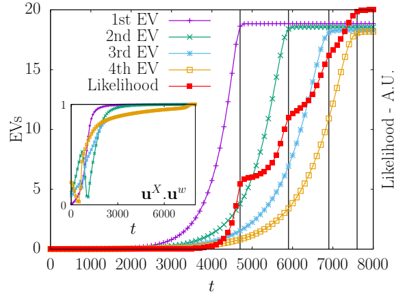
Fig. 4: Time evolution of the eigenvalues in the linear model and of the likelihood. We observe very clearly how the different modes emerge from the bulk and how the likelihood increases at each eigenvalue learned. In the inset, the scalar product of the vectors \mathbf{u} obtained from the SVD of the data and of \mathbf{w} . The \mathbf{u} s of \mathbf{w} are aligned with the SVD of the data at the end of the learning.
