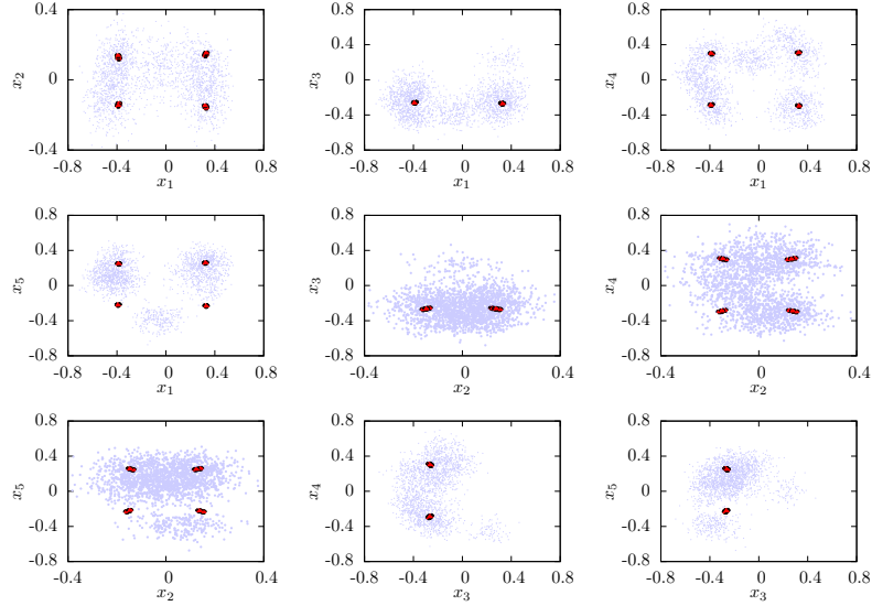
Fig. 6: Scatter plots of the mean-field magnetizations (in red) and the samples (in blue) in various planar projection defined by pairs of left eigenvectors of W . This case corresponds to an RBM of size (N_v, N_h) = (100, 50) learned on a synthetic data set of 10^4 samples of size N_v = 100 obtained from a multi modal distribution with 11 clusters randomly defined on a submanifold of dimension d = 5 . The scatter plot is obtained at a point where 5 modes have already condensed and 16 saddle point solutions have been found.
