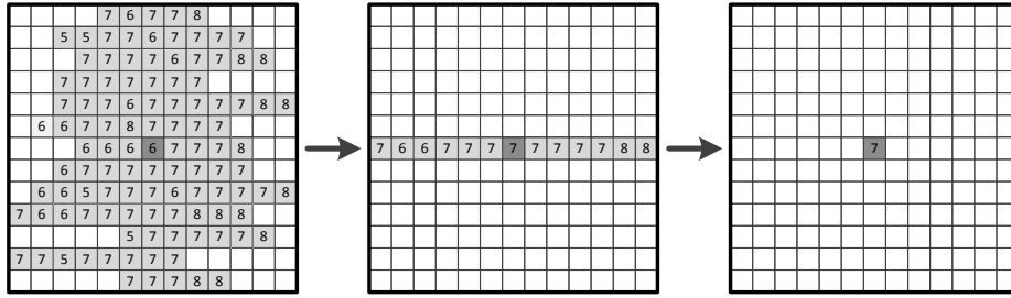
Fig. 4. The vertical-horizontal approach for disparity voting.
