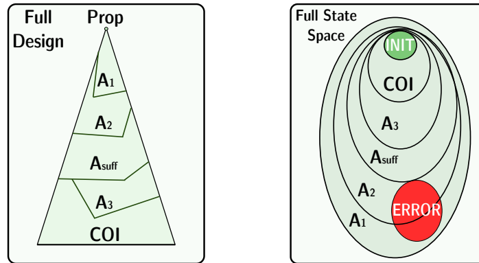
(a) Localization abstractions with different degrees of precision
