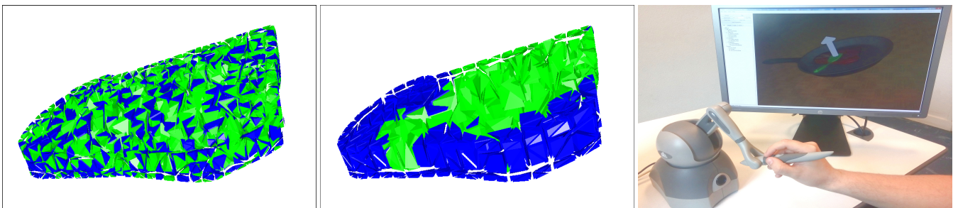
Figure 1: Overview of our elasticity-based clustering approach: (left) Based on an heterogeneous object composed of elements with different elasticity values, (center) we propose to build elasticity clusters to improve the computation time performances, (right) thus allowing haptic interaction while keeping similar perceptual sensations.
