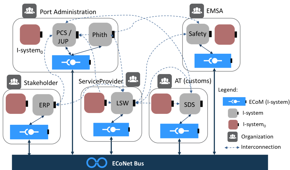
Fig. 4. – The collaborative network established by the LSW services
