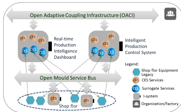
Fig. 2. The two-layered open service bus based on the CES model.
