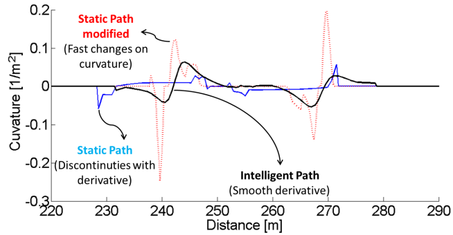
(c) Derivative of the curvature
