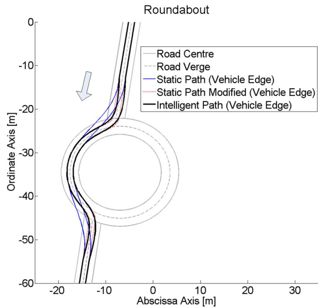
(a) Roundabout
