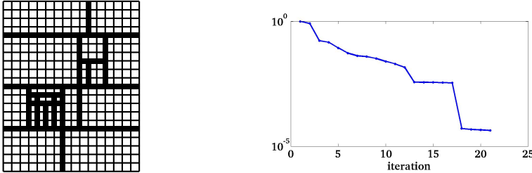
Figure 4.9: Test 2: strategy 1 when exact S and T have different zonations. Zonation after 21 iterations (left) and variation of the misfit function during the iterations (right).
