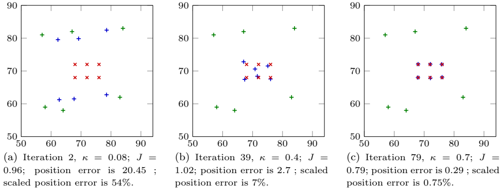
Figure 13: Obstacles position recovery using 23dB data with the SD2-LS2 method and starting from initial guess 2 (Figure 3(b)). Experiment [6Obs.23dB.IG2].
