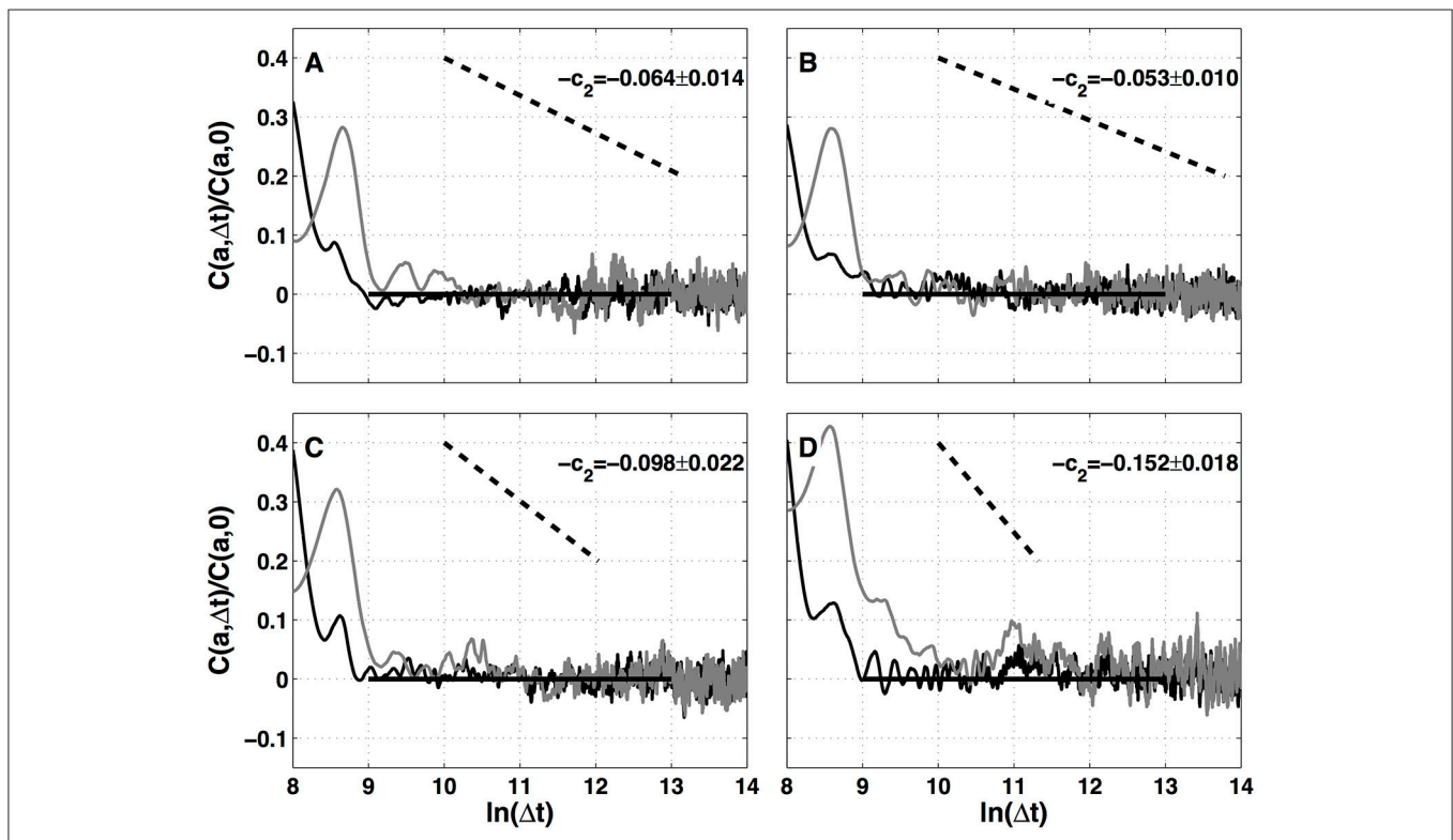
FIGURE 9 | Two-point magnitude analysis of local impulse energy time-series recorded along the CS vein. Two-point correlation function C(a, \Delta t)/C(a, 0) vs. \ln(\Delta t) (Equation 15) for local impulse energy E(t) computed with the analyzing wavelet g^{(3)} . The two curves correspond to scales a = 2^9 (black) and 2^{10} (gray) within the scaling range. (A) Pt1, (B) Pt2, (C) Pt3, and (D) Pt5.
