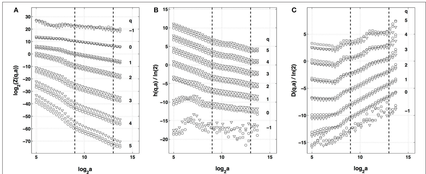
FIGURE 3 | Multifractal analysis of local impulse energy time-series recorded at the electrode Pt2 with the WTMM method. (A) \log_2 Z(q, a) vs. \log_2 a (Equation 3). (B) h(q, a) / \ln 2 vs. \log_2 a (Equation 5). (C) D(q, a) / \ln 2 vs. \log_2 a (Equation 6). The computation were performed for different values from q = -1 to 5 with the analyzing wavelet g^{(1)} ( \nabla ), g^{(2)} ( \square ) and g^{(3)} ( \circ ) (Figure S1). The vertical dashed lines delimit the range of scales ( 2^9 \leq a \leq 2^{13} ) used for the linear regression estimate of \tau(q) , h(q) and D(q) in Figure 4 .
