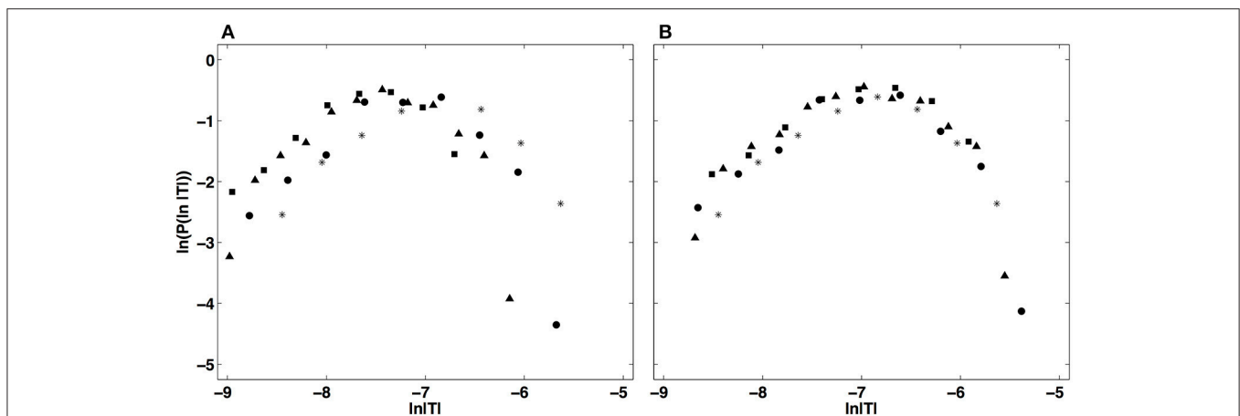
FIGURE 5 | Demonstration of the WTMM pdf rescaling via the propagative equation across scales (Equation 13). (A) Original pdfs of the logs of WTMM coefficients (magnitude coefficients) of the local impulse energy time series recorded at the electrode Pt2, computed with the analyzing wavelet g^{(3)} , at scales a (= \Delta t/\Delta t_0 , where \Delta t_0 = 10^{-4} s) = 2^9 (*), 2^{10} (●), 2^{11} (▲) and 2^{12} (■). (B) Rescaled pdfs using the multifractal quadratic estimate of the \tau(q) spectrum (Equation 10) with parameters [c_0, c_1, c_2] = [1.01, -0.34, 0.053] (see Table 1 ).
