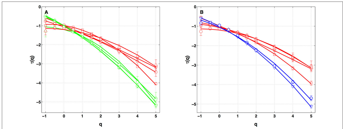
FIGURE 8 | \tau(q) spectra of local impulse energy time-series recorded along the CS vein at the electrodes Pt2 (red), Pt3 (blue) and Pt5 (green). The curves represent quadratic polynomial fit of the data (Equation 10). (A) The symbols correspond to the reference Patient 1 (chronic AF, \nabla ) and to Patients 2 (chronic AF, \circ ), 3 (paroxysmal AF, \square ) and 4 (persistent AF, \Delta ). (B) The symbols correspond to the reference Patient 1 ( \nabla ) and to three different time-series for Patient 4 ( \circ , \square , \Delta ) recorded at different periods of time preceding ablation procedure.
