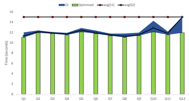
Figure 2: Comparing ranking-optimised query evaluation with other systems (SNB data 5M nodes)
