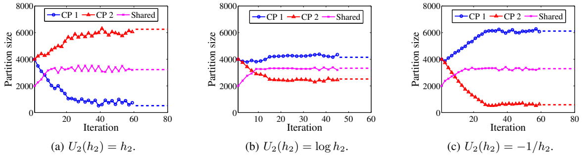
Fig. 13: Convergence of the online algorithm when some content is served by both content providers. U_1(h_1) = \log h_1 .
