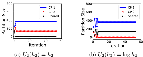
Fig. 15: Performance of the online algorithm over real-world trace with some content served by both providers. U_1(h_1) = h_1 .
