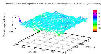
Figure 5: Lag plot for Synth. \rho = 100|1\%|3 - 5 .
