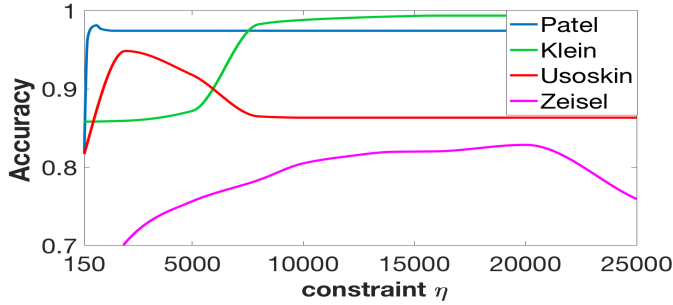
Fig. 7: Selection of the optimal \ell^1 bound, \eta_{opt} . A typical behaviour on biological applications is the existence of a plateau-like zone: if \eta too big, too many genes are selected (including irrelevant ones for the clustering) by the presence of technical and biological noise in their expression, which reduces accuracy. Conversely, for \eta too small, not enough information is available and the accuracy of clustering is also reduced.
