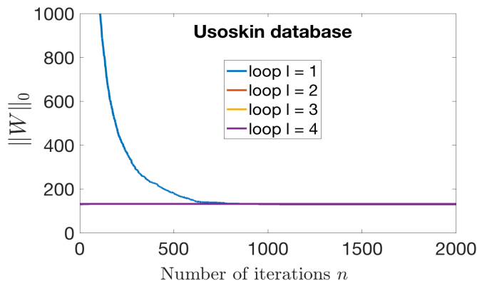
Fig. 3: Evolution of \|W\|_0 on Usoskin database versus the number of iterations. The number of nonzero entries of the sparse matrix W depends on the sharpness of the \ell^1 constraint (5) defined by \eta , and on the iteration n . (As n ranges from 0 to N , sparsity is increased rapidly in the first loop).
