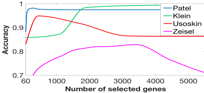
Fig. 8: Accuracy versus number of genes. These results show that a minimum number of genes is required to get the best possible clustering accuracy. Such genes are involved in the most relevant biological processes necessary to distinguish cell types. On the one hand, on Patel and Klein datasets, an increasing number of genes used for clustering between conditions will only add repetitive signal to the minimum number of genes necessary, and will neither increase nor decrease the clustering accuracy. On the other hand, on Zeisel and Usoskin datasets, adding too many genes would result in a decrease in clustering accuracy. Implying that the additional genes are noisy due to technical and biological variations with little relevance to distinguish between cell types.
