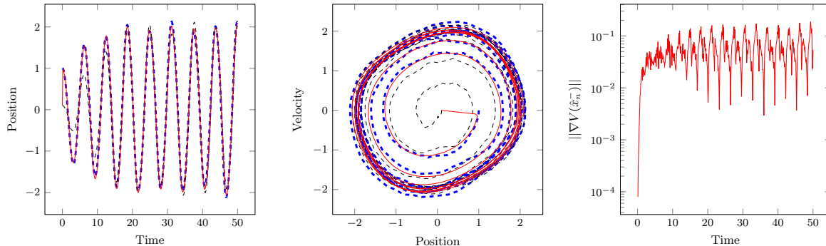
FIGURE 6. Trajectory (left) and Phase portrait (middle) of the target trajectory (blue, dashed), the estimator (red), and the uncorrected trajectory (black dashed). Optimality verification from the time plot of \|\nabla V(\hat{x}_n^-)\| (right)
