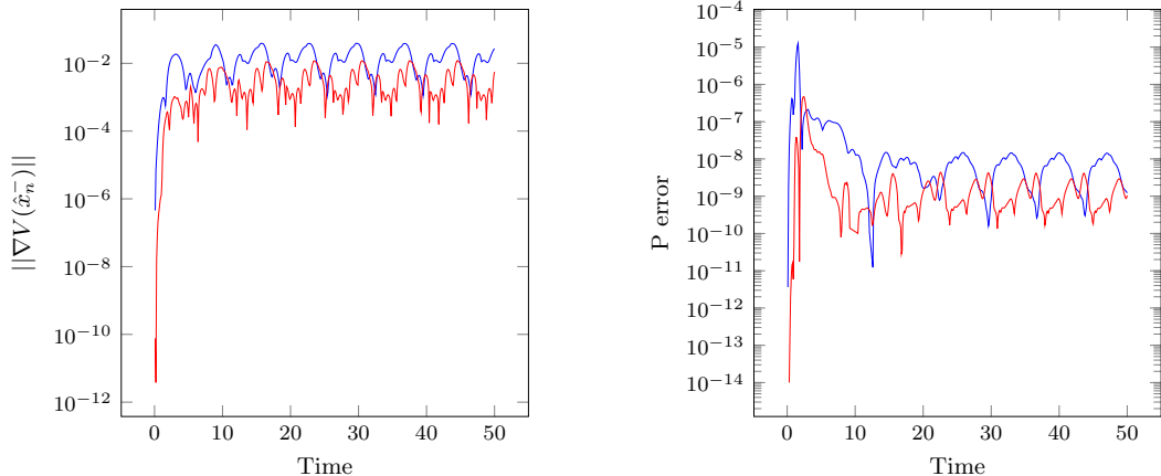
FIGURE 5. Optimality verification from the time plot of \|\nabla\mathcal{V}^-(\hat{x}_n^-)\| (left) and Covariance computation verification with discrete-time Riccati solution (right). 10x10 discretization (blue) and 20x20 discretization (red)
