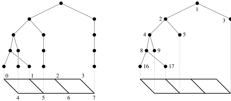
a. Recursive coarsening tree obtained from Figure 3. b. Derived recursive bipartitioning tree.
