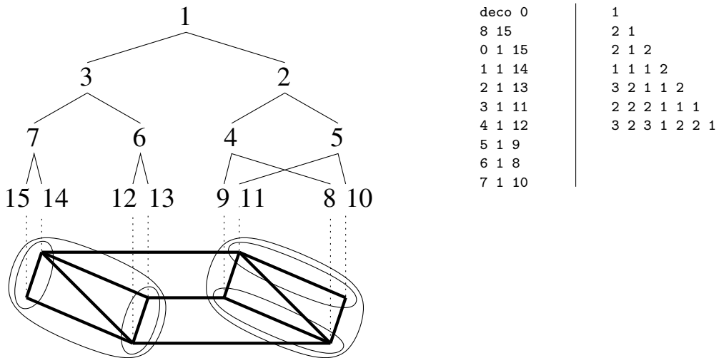
a. Recursive coarsening tree of UB(2, 3) .
