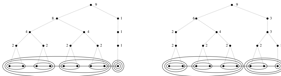
a. Matching starting from the leftmost vertex only. b. Matching starting alternatively from the leftmost and rightmost vertices.
