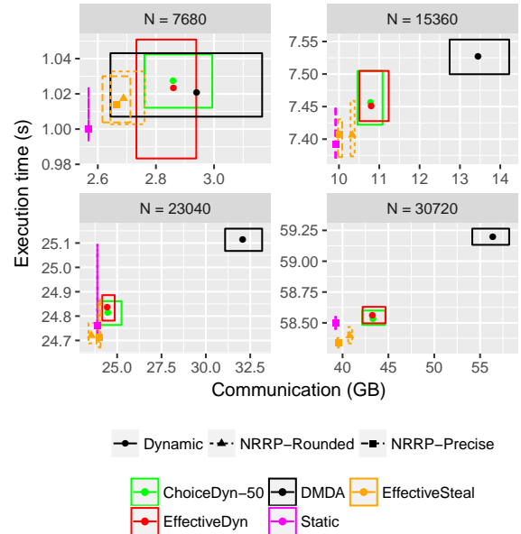
Figure 8: Execution time and communication results on the mirage platform.
